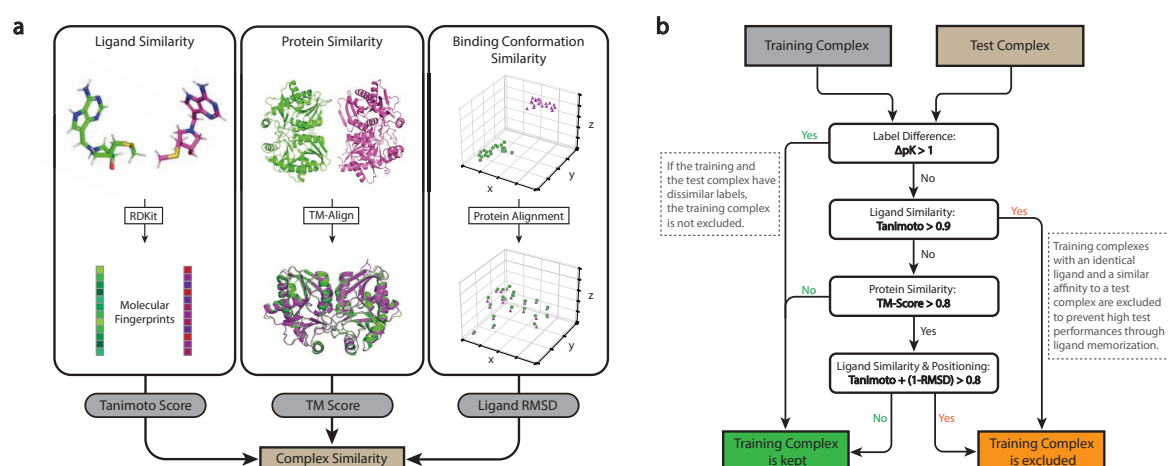
Figure 1: Overview of the Similarity Computation Between Two Protein-Ligand Complexes: a) Our structure-based dataset filtering algorithm evaluates structural similarity of protein-ligand complexes using a combination of protein similarity (TM-scores), ligand similarity (Tanimoto scores) and binding conformation similarity (pocket-aligned ligand RMSD). The Tanimoto scores identify chemically similar ligands and range from 0 (no similarity) to 1 (identical). TM-scores are computed with TM-align, a tool that compares protein structures by finding the optimal alignment of their three-dimensional structures and outputs a score ranging from 0 (no similarity) to 1 (identical). This score identifies proteins with high structural similarity, even when sequence identity is low (e.g. when one protein is a substructure of the other). Pocket-aligned ligand RMSD scores compare the positioning of ligands within aligned protein pockets. Ligands are transformed into the same coordinate frame using the optimal alignment from TM-align, and a root-mean-square-deviation (RMSD) calculation provides a quantitative measure of positional similarity. b) Decision tree showing the exclusion criteria and the information flow of the filtering algorithm when comparing a training and a test complex. The first layer of the algorithm compares the affinity labels of the complexes (pK values, see Methods). Training complexes with high structural similarity but different activity are not excluded, to avoid excluding data points that can provide valuable insights into activity cliffs. The second layer excludes all training complexes with similar affinity and identical ligand (Tanimoto > 0.9) to make the test complex ligands unique and avoid successful predictions through ligand memorization. The third and fourth layer exclude training complexes based on protein similarity and a combined assessment of ligand and binding conformation similarity. This four-layer approach identifies complexes with similar interaction patterns, even when traditional sequence-based methods would overlook these similarities.
