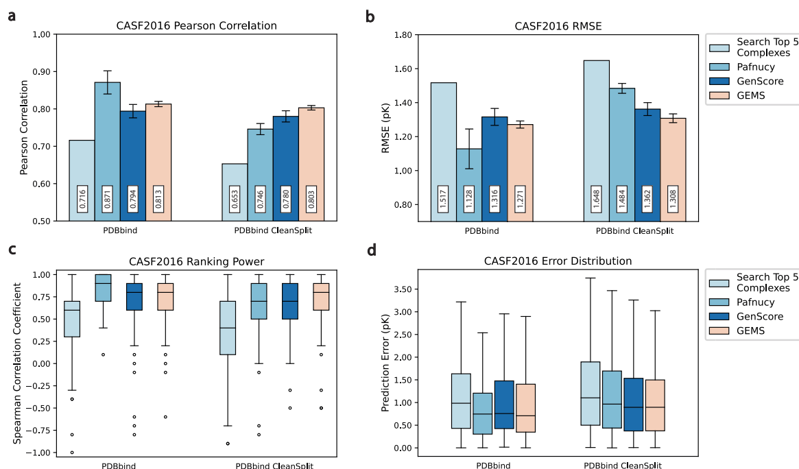
Figure 3: Prediction Accuracy of GEMS, Pafnucy and GenScore in Dependence of Dataset Filtering: a) CASF2016 Pearson correlation coefficients of a simple search algorithm (Search Top 5 Complexes), Pafnucy, GenScore, and GEMS when trained on the original PDBbind dataset (left) and the filtered PDBbind CleanSplit dataset (right). b) CASF2016 prediction RMSE values of a simple search algorithm (Search Top 5 Complexes), Pafnucy, GenScore and GEMS when trained on the original PDBbind dataset (left) and the filtered PDBbind CleanSplit dataset (right). c) Ranking power: The distribution of Spearman correlation coefficients for the search algorithm, Pafnucy, GenScore and GEMS across all 57 clusters of CASF2016, presented separately for training on PDBbind (left) and PDBbind CleanSplit (right). d) Distribution of prediction errors (pK unit) across all CASF2016 complexes shown for a simple search algorithm (Search Top 5 Complexes), Pafnucy, GenScore, and GEMS when trained on the original PDBbind dataset (left) and the filtered PDBbind CleanSplit dataset (right). For each Pafnucy, GenScore and GEMS, five models were trained with five different train-validation splits. The performance values in a) and b) reflect the mean CASF2016 performance of the five models, with error bars representing the standard deviation across the performance of the five models. To compute the distributions of the Spearman correlation coefficients and prediction errors in c) and d) , the predictions of the five models were averaged into an ensemble prediction.
