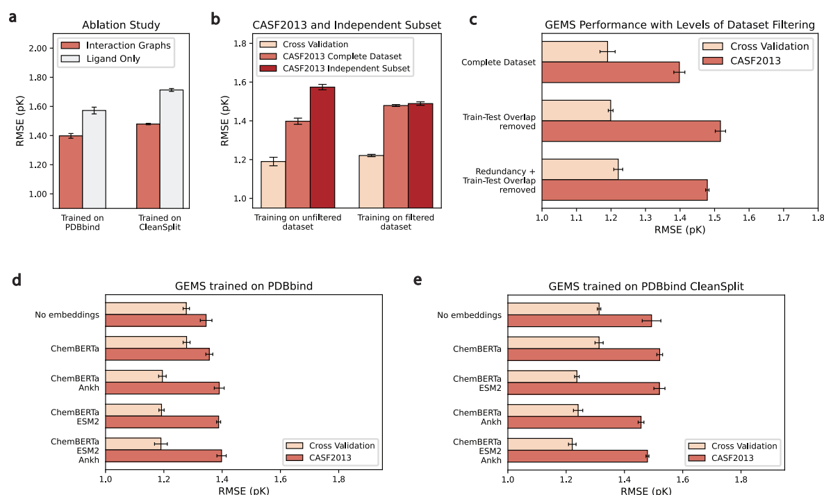
Extended Data Figure 4: Impact of Ablation and Dataset Filtering on GEMS Performance on CASF2013 (N=195): a ) Ablation study showing the impact of removing all protein information from the graphs on CASF2013 performance, comparing models trained on PDBbind (left) and PDBbind CleanSplit (right). b ) Comparison of GEMS performance on cross-validation (CV), CASF2013, and the independent subset of CASF2013 (N=89), for models trained on PDBbind (left) and PDBbind CleanSplit (right). c ) CASF2013 performance of GEMS with varying levels of training dataset filtering: complete dataset (PDBbind), train-test overlap removed, and both overlap and redundancy removed (PDBbind CleanSplit). Error bars represent data uncertainty, calculated as the standard deviation of the performance across five models trained with 5-fold cross-validation at different random seeds. d ) Effect of incorporating language model embeddings on the cross-validation and CASF2013 (n=285) performance of GEMS models trained on the original PDBbind dataset. e ) Effect of incorporating language model embeddings on the cross-validation and CASF2013 (n=285) performance of GEMS models trained on the PDBbind CleanSplit.
