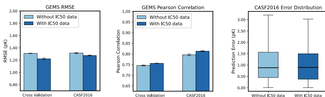
Extended Data Figure 2: Performance of GEMS with and without IC50-labeled complexes: Comparison of cross validation and CASF2016 (N=285) prediction accuracy of GEMS in terms of a ) RMSE, b ) Pearson correlation and c ) absolute prediction errors depending on inclusion of 6400 complexes labeled with IC50 values in the training data. Performance values represent the mean values of five models trained with 5-fold cross-validation at different random seeds. Error bars represent data uncertainty, calculated as the standard deviation of the performance across the five models
