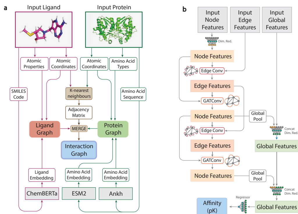
Figure 4: Graph-Based Modeling of Protein-Ligand Interactions and GEMS Model Architecture. a) Schematic overview of the graph construction process used to model protein-ligand complexes in a sparse, rotation- and translation-invariant graph representation enhanced with language model embeddings. The core of these graph representations consists of an atom-level molecular graph of the ligand molecule (magenta) combined with an amino acid-level graph of the protein pocket (green). During the merging of ligand and protein graphs, additional edges are introduced to connect ligand graph nodes (atoms) to protein graph nodes (amino acids) based on spatial proximity between ligand atoms and the atoms of the amino acids (interaction distance of 5Å), computed using a K-nearest neighbors algorithm. The amino acid nodes are featured with their type and embeddings derived from the protein language models ESM2 [50] and Ankh [51]. The ligand graph is featured with atomic properties. The global features are initialized with a ligand embedding from the language model ChemBERTa-2 [52]. b) GEMS model architecture for processing interaction graphs composed of node features, edge features, and global context features. After an initial node feature dimensionality reduction (Dim.Red.), node and edge features are transformed through an alternating sequence of node convolutions (GATConv) and edge convolutions (EdgeConv). The global graph features are dynamically updated throughout this process, incorporating pooled node representations after each node convolution. A final pK value prediction is made from the updated global features using a fully connected neural network.
