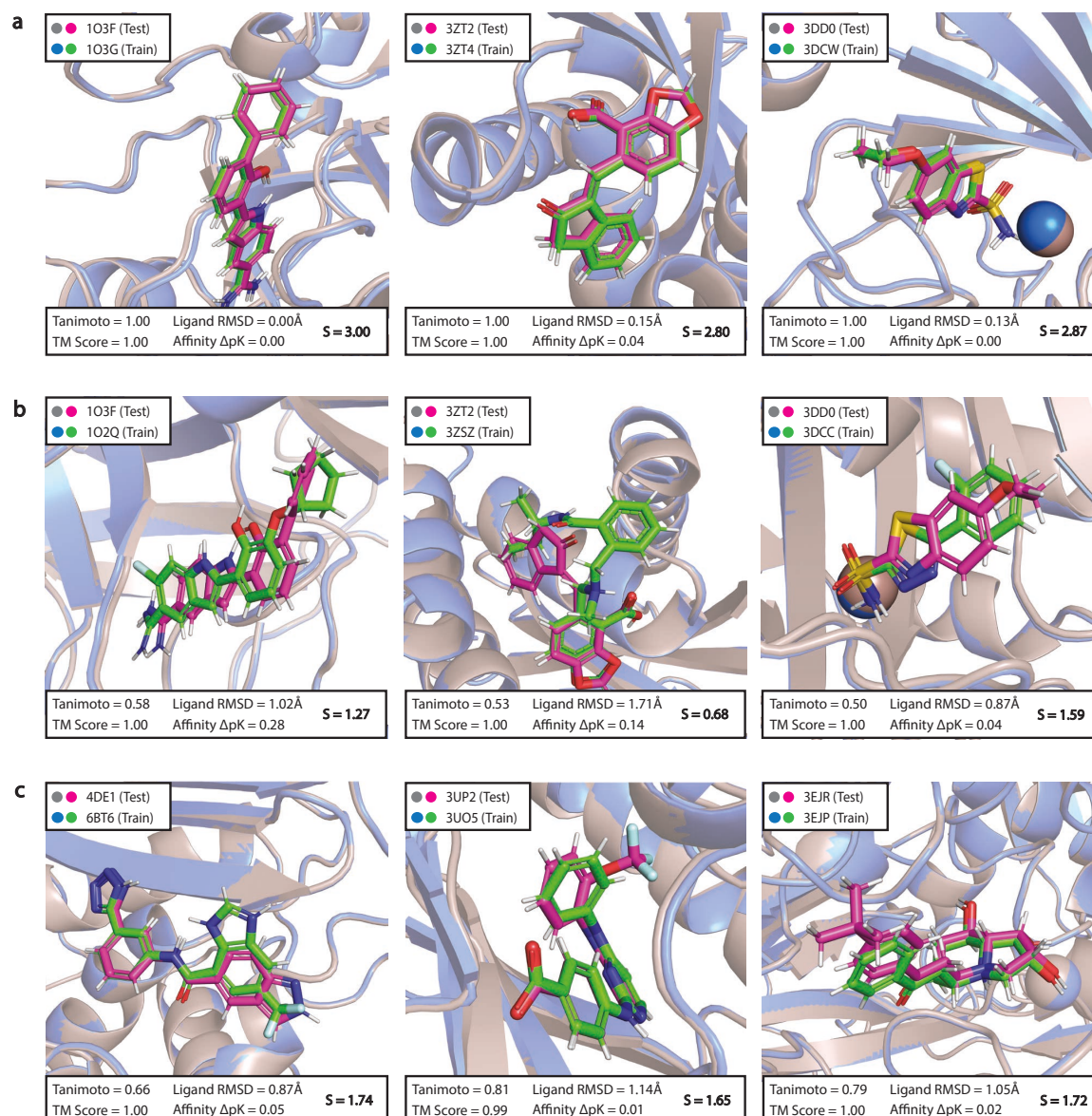
Figure 2: Superpositions of Complexes Highlighting Train-Test Structural Similarities Before and After Filtering: a) Superpositions of the most prominent train-test similarities before applying the filtering algorithm. b) Superpositions of the same test complexes as in a) , now shown with the most similar training complexes found in PDB CleanSplit. c) Superpositions of the closest train-test similarities that remained post-filtering in the dataset PDBbind CleanSplit. Protein structures from the test and training datasets are depicted as grey and blue cartoons, respectively, with ligands shown in magenta (test) and green (train). Below each superposition, the Tanimoto score, TM-score, ligand RMSD, and affinity difference ( \Delta pK ) is shown, which are combined into an overall similarity score S = \text{TM-Score} + \text{Tanimoto} + (1 - \text{Ligand RMSD}) - \Delta pK . This S -score was computed for all possible train-test pairs and served to select representative complexes for this figure. For each training dataset, the depicted pairs were selected from the top 5 pairs with the highest S , prioritizing good ligand visibility. In some superpositions (103F/103G and 3DD0/3DCW), one structure has been slightly shifted to enhance visibility of structural differences. Original PyMol sessions of all of superpositions are provided on GitHub.
